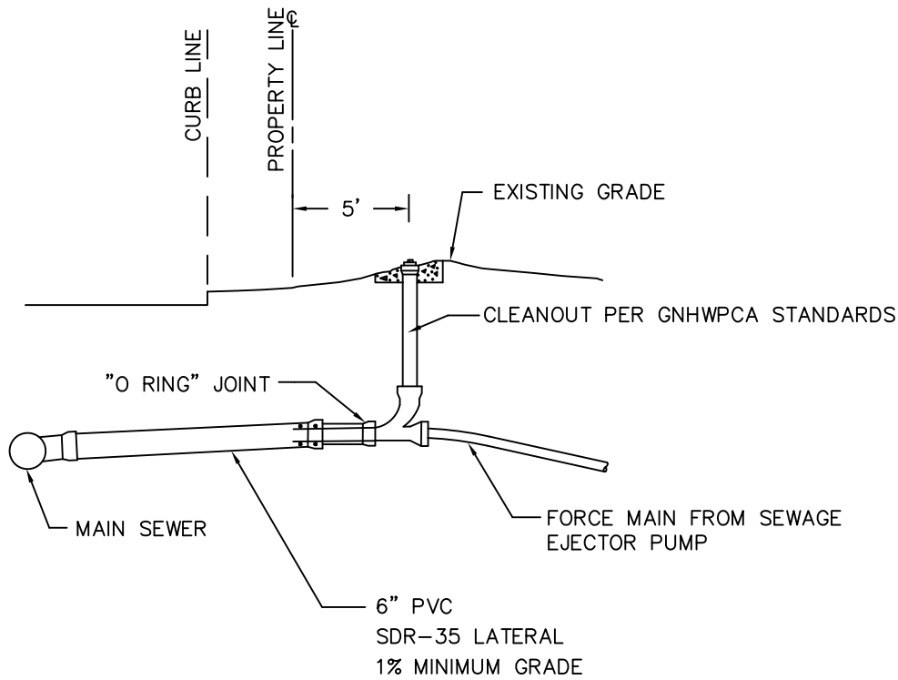
PROFILE
