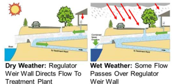
Combined Sewer Overflow (CSO) Diagram
