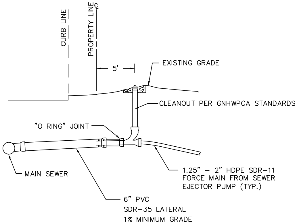
PROFILE
