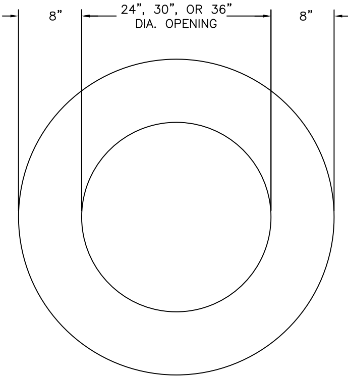
GRADE RING PLAN VIEW
