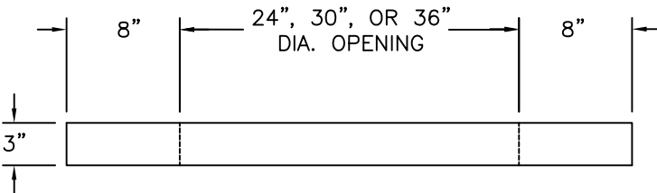
GRADE RING ELEVATION VIEW
